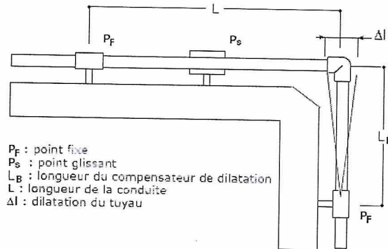
Figure 5 : Supports mobiles
