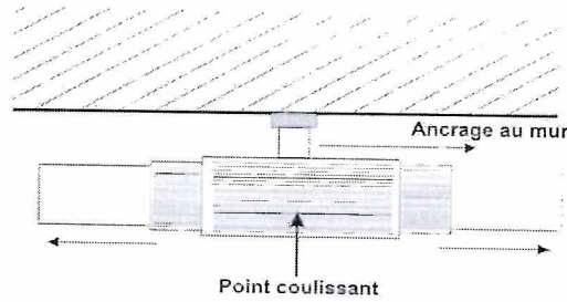
Figure 5 : Supports mobiles
